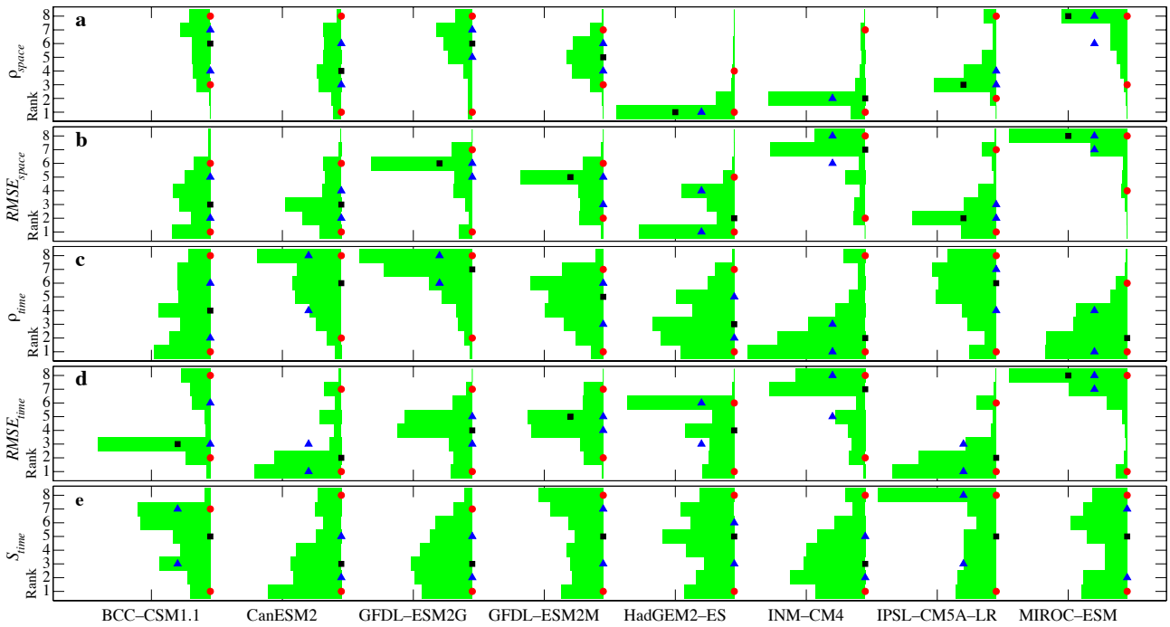
Figure 3. Skill rank by model. Histograms for ranked (a) spatial correlation, \rho_{space} ; (b) spatial RMSE, RMSE_{space} ; (c) temporal correlation, \rho_{time} ; (d) temporal RMSE, RMSE_{time} ; and (e) distributional similarity, S_{time} . Lower ranks denote relatively higher levels of model–data agreement. Distributions are displayed as horizontal histograms and share the same scale within each panel. Colored symbols give percentiles. Median, black square; interquartile range (25–75 percentiles), blue triangles; and 2.5–97.5 percentiles, red circles. Some symbols jittered to avoid overlap.
